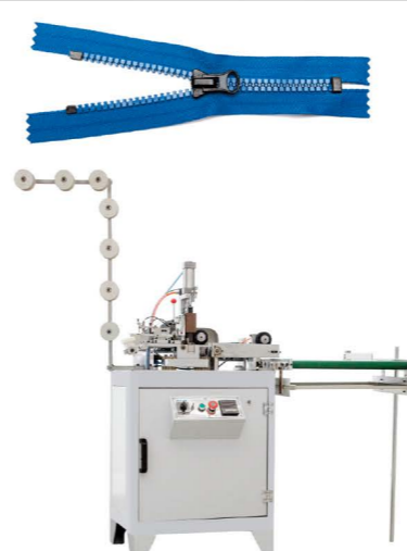
QLQ-ZCM-1 Automatic Plastic Zipper Closed-end Zigzag Cutting M/C
