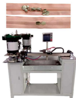
QLQ-DSMCM Automatic Zipper Double Sliders Mounting & Cutting Machine
