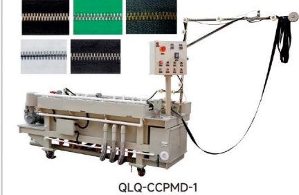
QLQ-CCPMD-1 Automatic Metal Zipper Chemical Cold Plating Machine (with two chemical tanks) (about 800-1200M/H)
