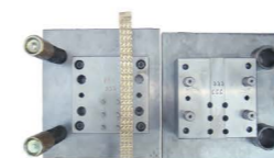
Slider Needle/Monkey Mould (C shape, 6 cavities)
