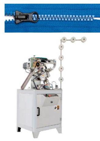
QLQ-SMM Automatic Plastic Zipper Slider Mounting M/C (for normal type bottom stop)
