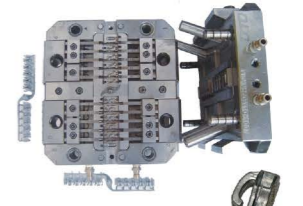
N56 Non-lock Reverse Slider Body Mould
