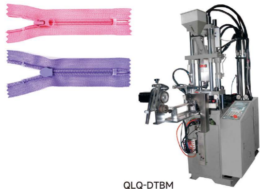
QLQ-DTBM Automatic Zipper Closed-end Injection M/C
