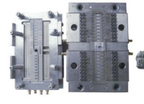
N31A Spring-lock Slider Body Mould
