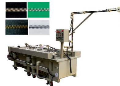
QLQ-CCPMS-1 Automatic Metal Zipper Chemical Cold Plating Machine (with one Chemical Tank) (about 800-1200M/H)
