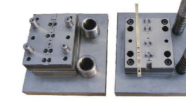
Pressing Puller Mould
