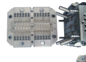
N53 Pin-lock Slider Body Mould
