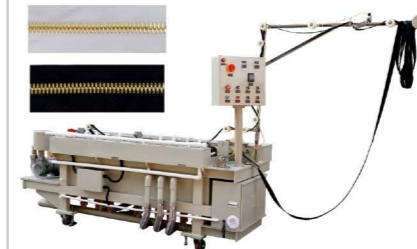
QLQ-GPM-1 Automatic Metal Zipper Shiny Gold Plating Machine (about 800-1200M/H)
