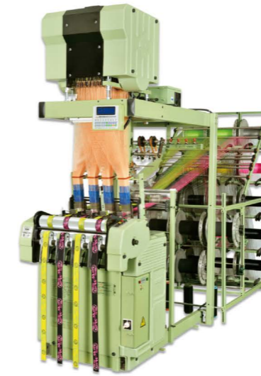
QLQ-CJM-1 Computerized Jacquard Machine (made in China)
