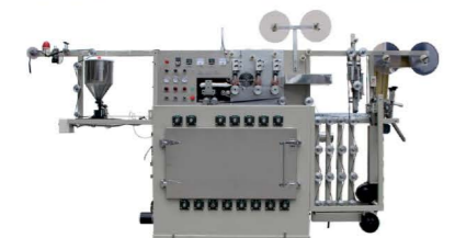
QLQ-WZGFSM Automatic Waterproof Zipper Gumming & Film Sealing Machine (2 in 1 model, PVC/TPU/PU available)
