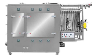
QLQ-NIIM-2 Automatic Nylon & Invisible Zipper Ironing Machine (new type, two chambers)
