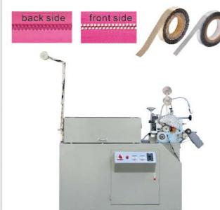
QLQ-PSFSM-1 Automatic Plastic Zipper Shiny Film Sealing Machine (old model)
