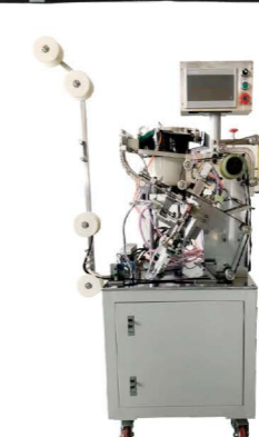
QLQ-SMM-2 Automatic Plastic Zipper Single Side Slider Mounting M/C (side mounting model)
