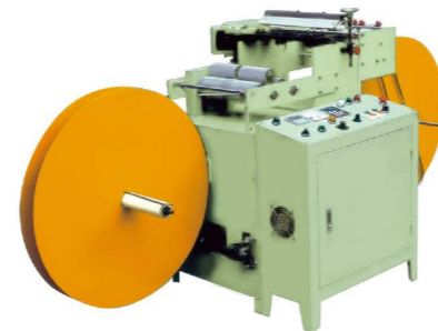
QLQ-VHCM Velcro Hook Cutting Machine
