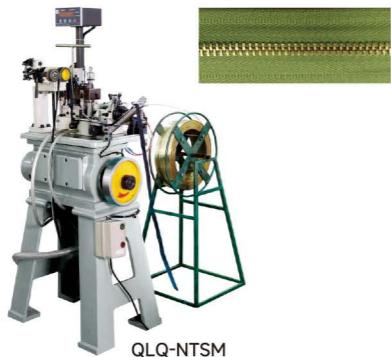
QLQ-NTSM Automatic Metal Zipper Normal Teeth Stamping Machine
