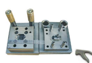
Slider Needle/Monkey Mould (Y shape, 3 cavities)
