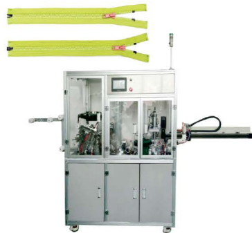
QLQ-SCBM Automatic Plastic Zipper Slider Mounting & Ultrasonic Cutting & Box Fixing M/C (3 in 1)
