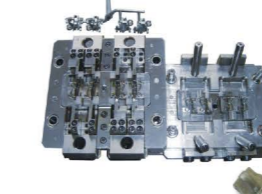
N106 Keyhole Non-lock Slider Body Mould
