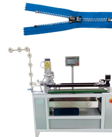
QLQ-ZCM-4 Automatic Plastic Zipper Ultrasonic Closed-end Zigzag Cutting M/C (with labour hand)
