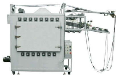
QLQ-4ZTIM/QLQ-6ZTIM Automatic Zipper Tape Ironing Machine (4 tapes/6 tapes, one chamber)
