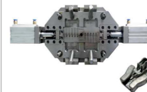
Invisible Slider Body Mould
