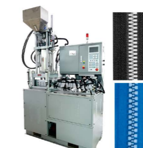
QLQ-DTM Automatic Plastic Zipper Teeth Injection Machine
