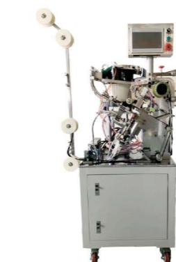
QLQ-SMM-2 Automatic Metal Zipper Single Side Slider Mounting M/C (side mounting model)
